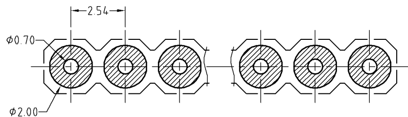
Recommended pcb layout Layout tolerance: ±0.05mm
