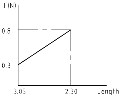
Spring force-Length
