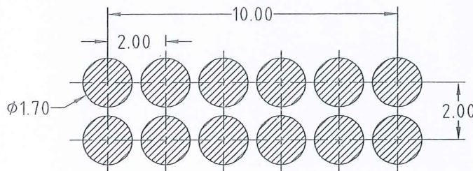
Recommended pcb layout Layout tolerance: ±0.05mm
